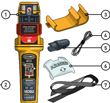
MOB2 Class M PLD All-Net Short-Burst Personal Locator Beacon with AIS
