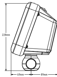
Horizontal Rail
